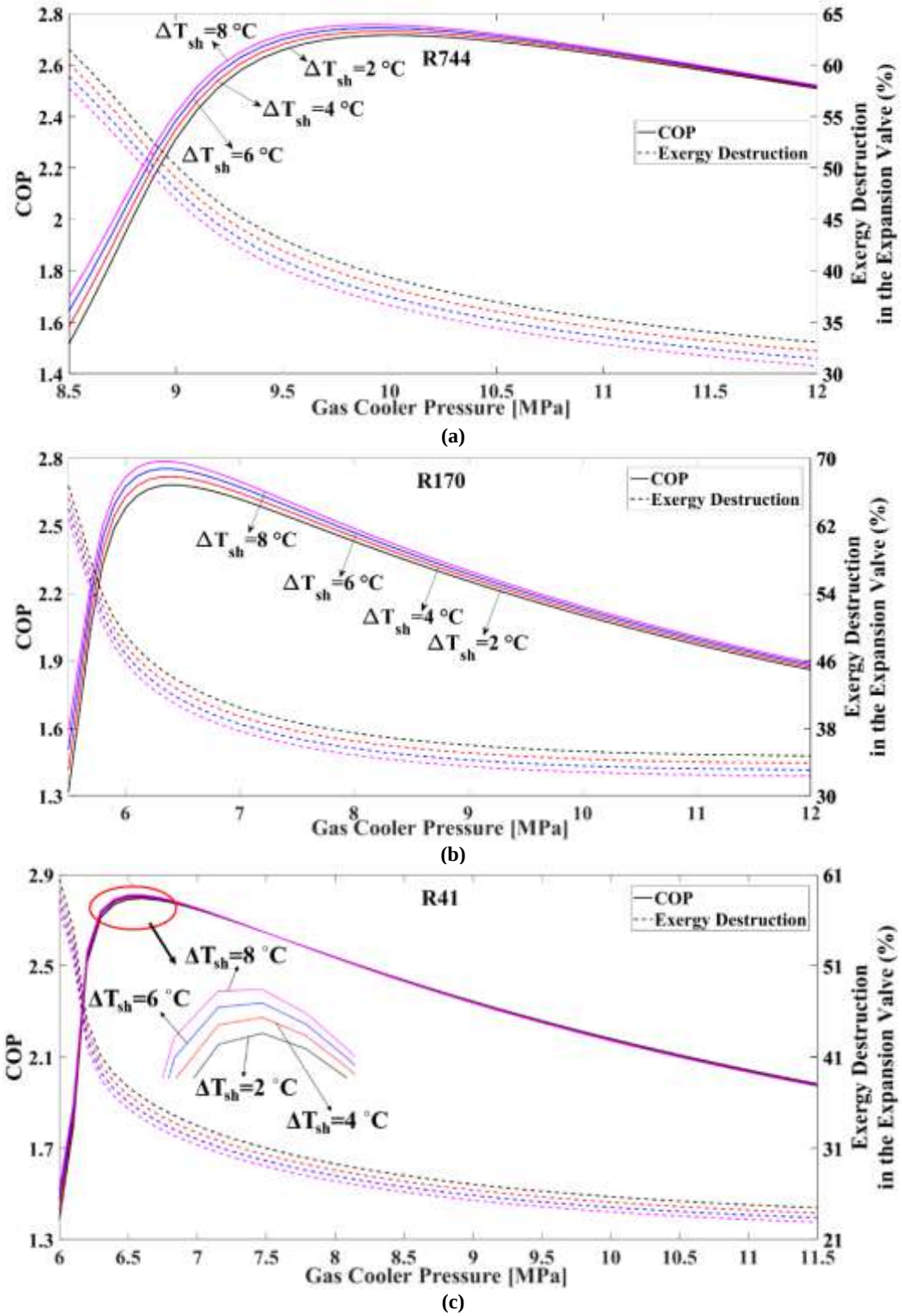
Figure 6. Effects of the evaporator outlet superheat temperature difference on the performance and percentage expansion losses based on the gas cooler pressure for R744 (a), R170 (b), and R41 (c).
